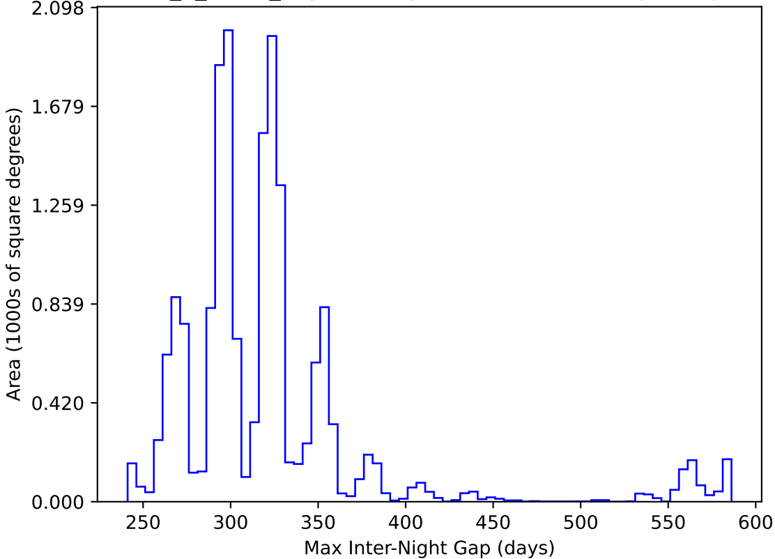
too_5_4v3.4_10yrs WFD y band: Max Inter-Night Gap
