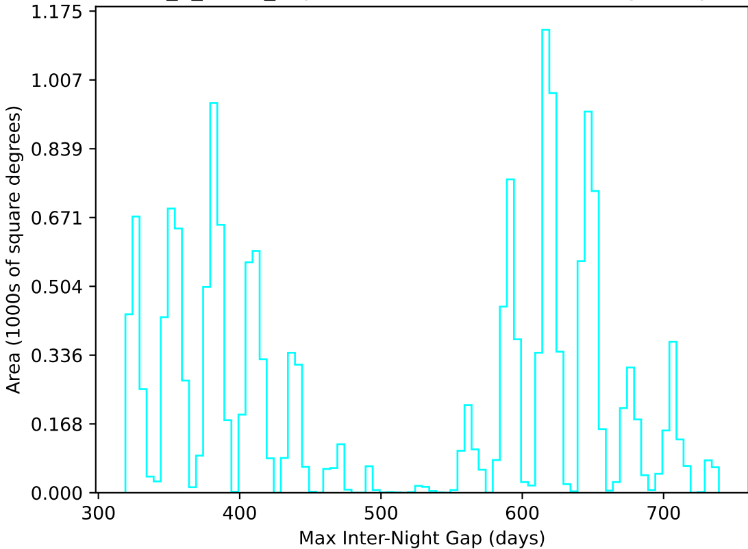
too_5_4v3.4_10yrs WFD u band: Max Inter-Night Gap
