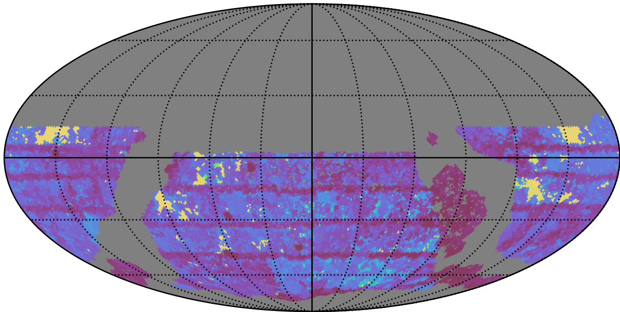
too_5_4v3.4_10yrs WFD r band: Max Inter-Night Gap
