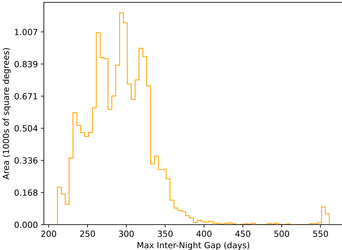
too_5_4v3.4_10yrs WFD r band: Max Inter-Night Gap
