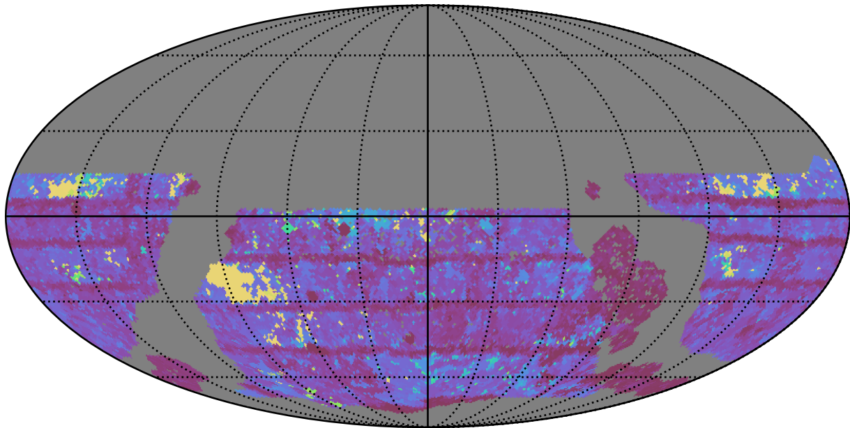
too_5_4v3.4_10yrs WFD i band: Max Inter-Night Gap
