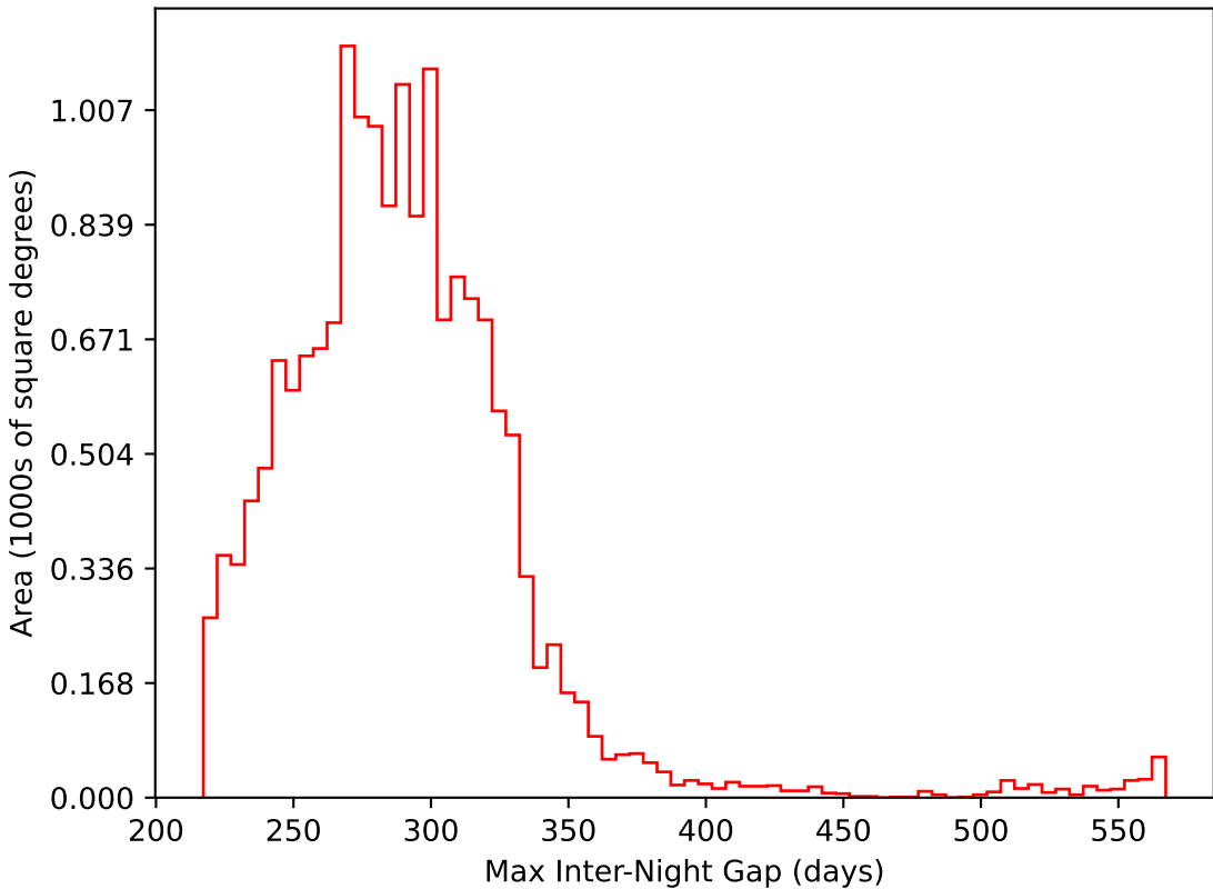
too_5_4v3.4_10yrs WFD i band: Max Inter-Night Gap
