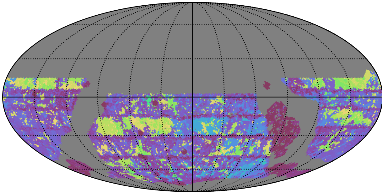
too_5_4v3.4_10yrs WFD g band: Max Inter-Night Gap
