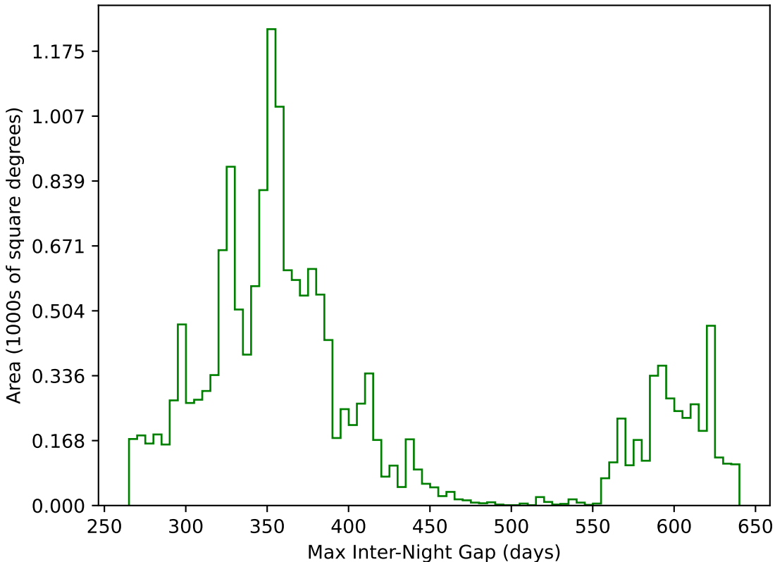
too_5_4v3.4_10yrs WFD g band: Max Inter-Night Gap
