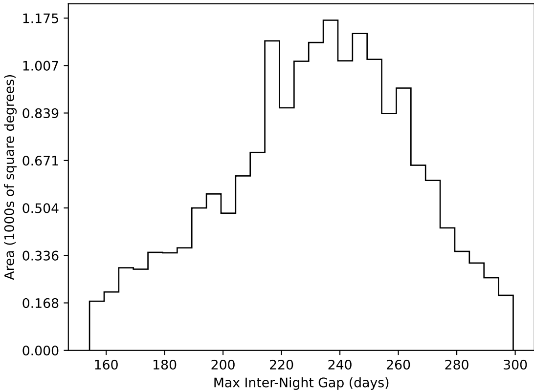
too_5_4v3.4_10yrs WFD all bands: Max Inter-Night Gap
