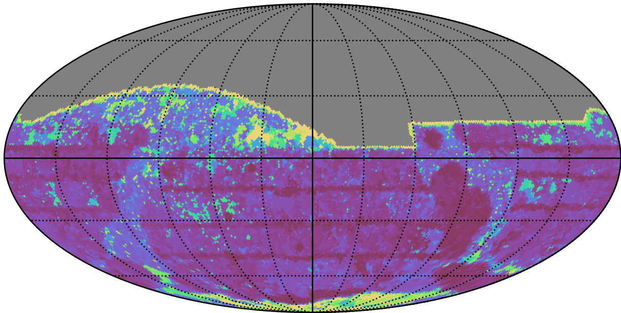
too_5_4v3.4_10yrs All sky z band: Max Inter-Night Gap
