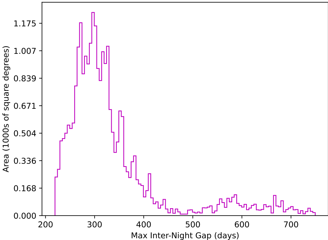
too_5_4v3.4_10yrs All sky z band: Max Inter-Night Gap
