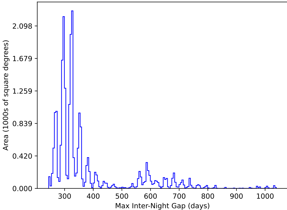
too_5_4v3.4_10yrs All sky y band: Max Inter-Night Gap
