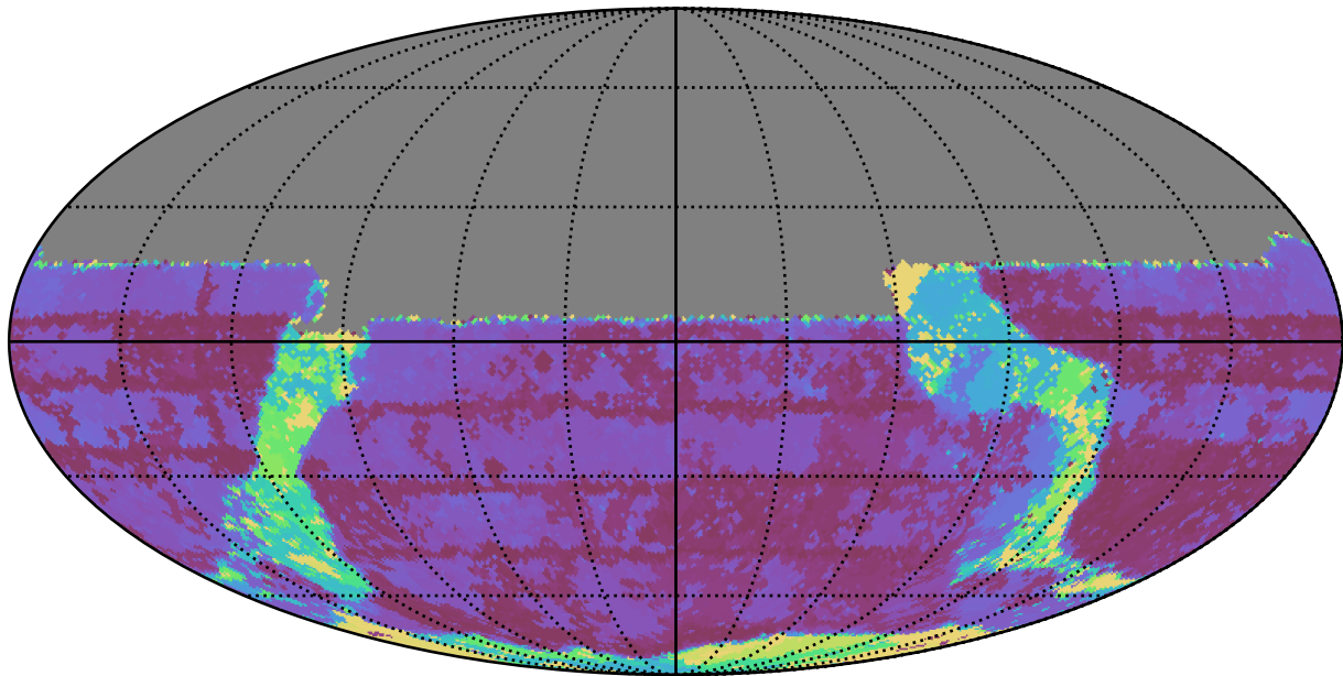
too_5_4v3.4_10yrs All sky u band: Max Inter-Night Gap
