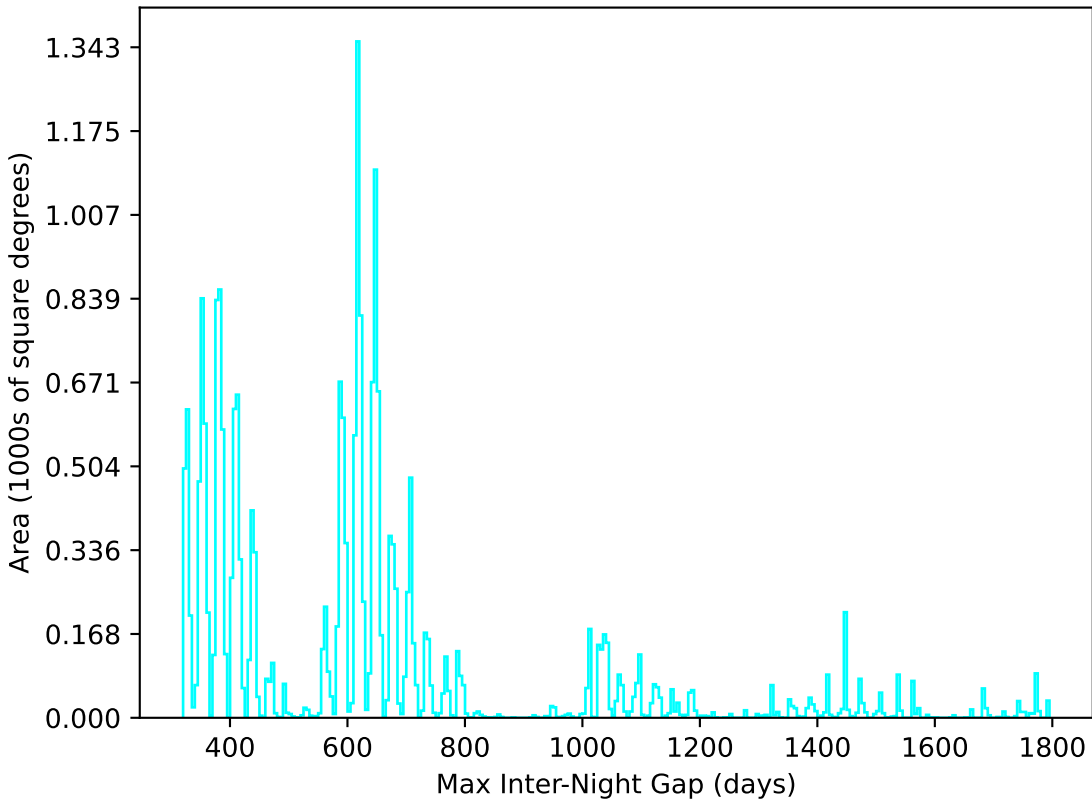
too_5_4v3.4_10yrs All sky u band: Max Inter-Night Gap
