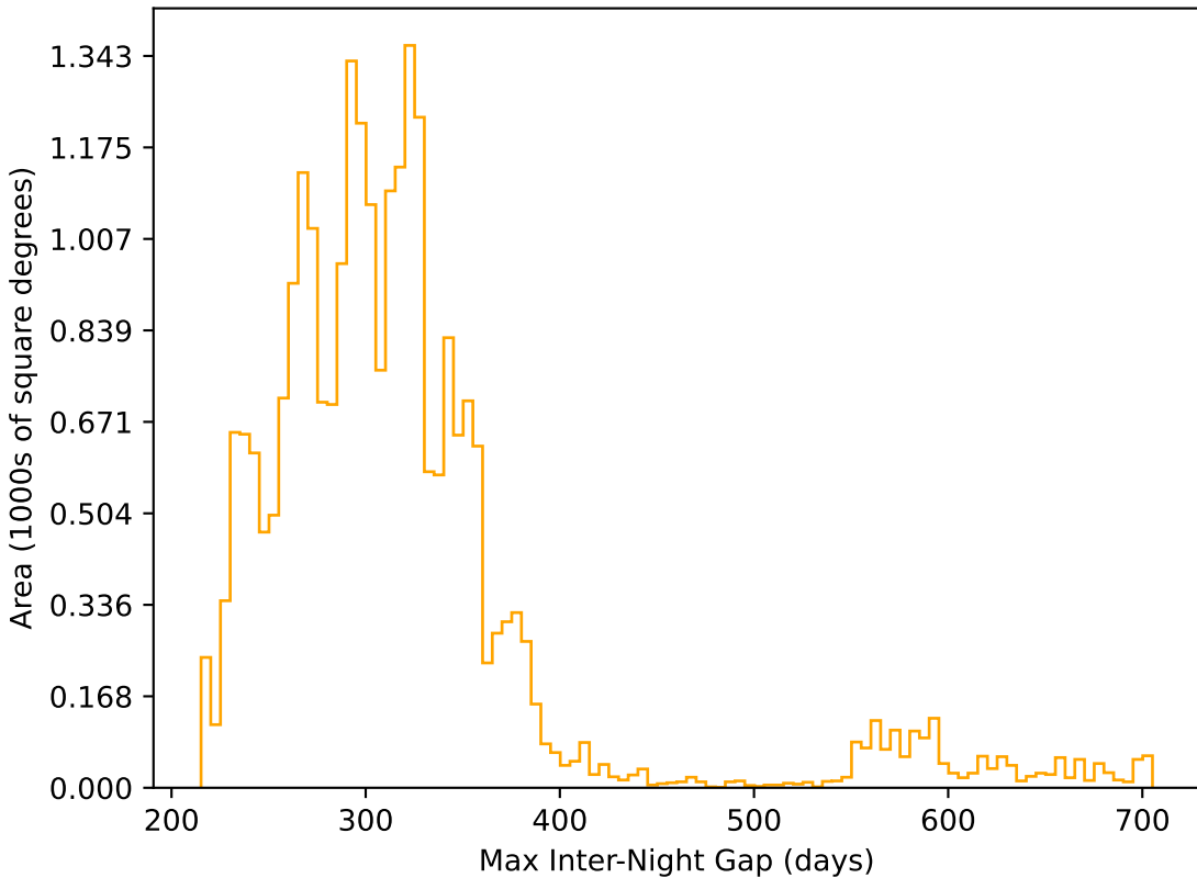
too_5_4v3.4_10yrs All sky r band: Max Inter-Night Gap
