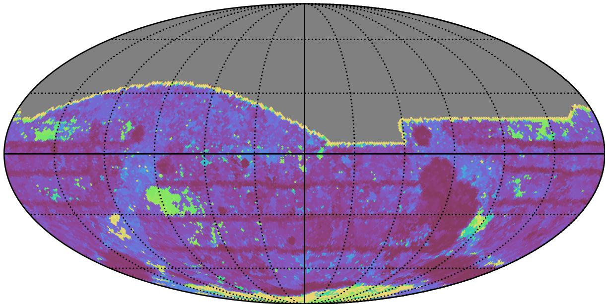
too_5_4v3.4_10yrs All sky i band: Max Inter-Night Gap
