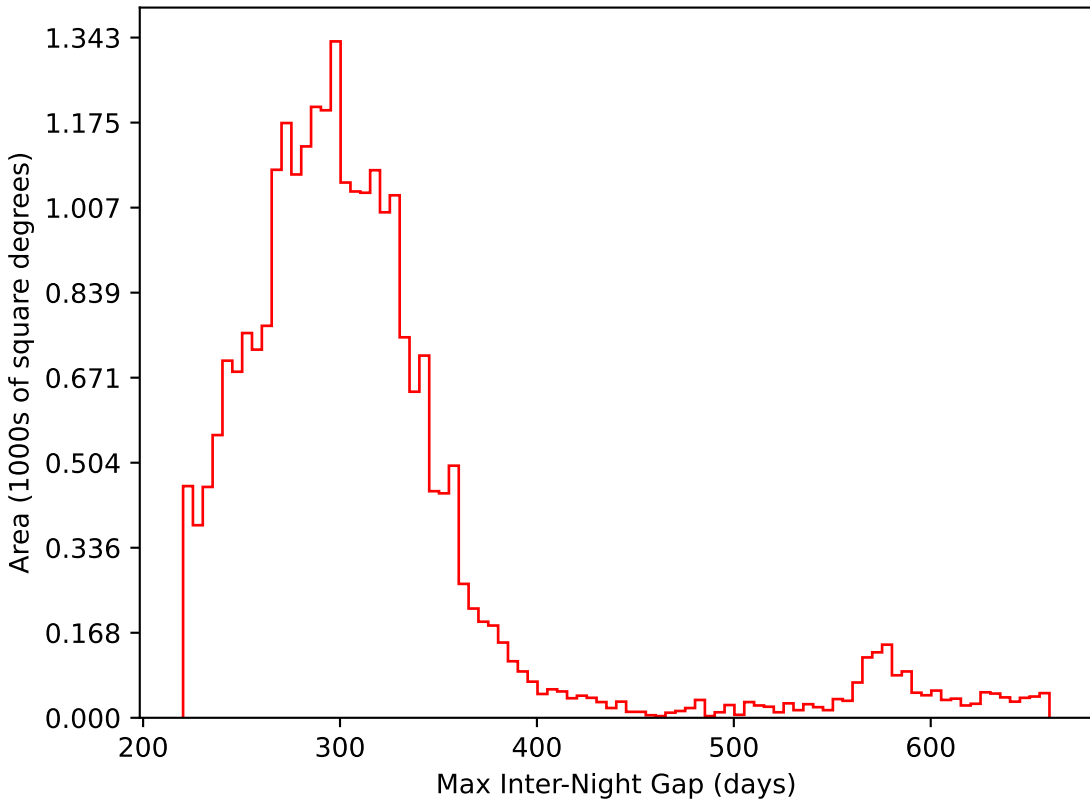
too_5_4v3.4_10yrs All sky i band: Max Inter-Night Gap
