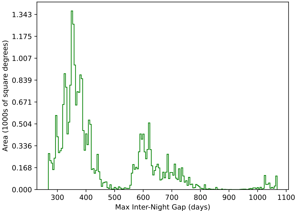
too_5_4v3.4_10yrs All sky g band: Max Inter-Night Gap
