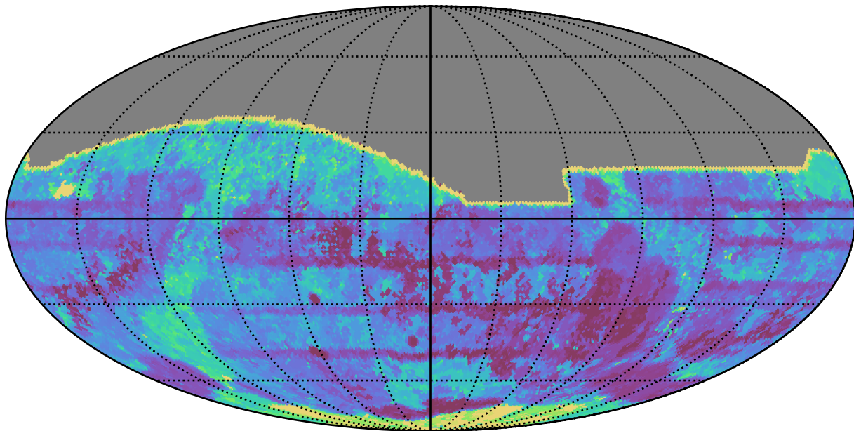
too_5_4v3.4_10yrs All sky all bands: Max Inter-Night Gap
