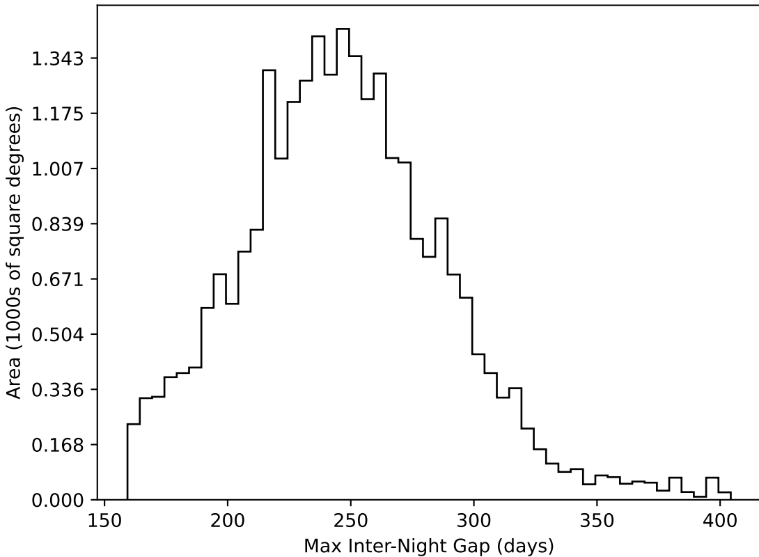
too_5_4v3.4_10yrs All sky all bands: Max Inter-Night Gap
