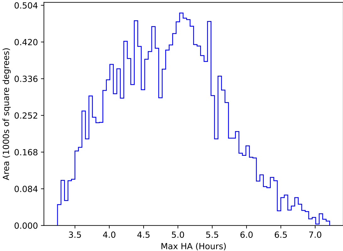
too_5_4v3.4_10yrs WFD z band: Max HA
