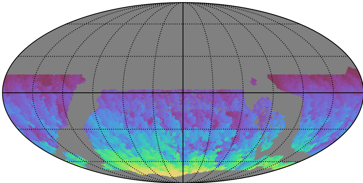
too_5_4v3.4_10yrs WFD y band: Max HA
