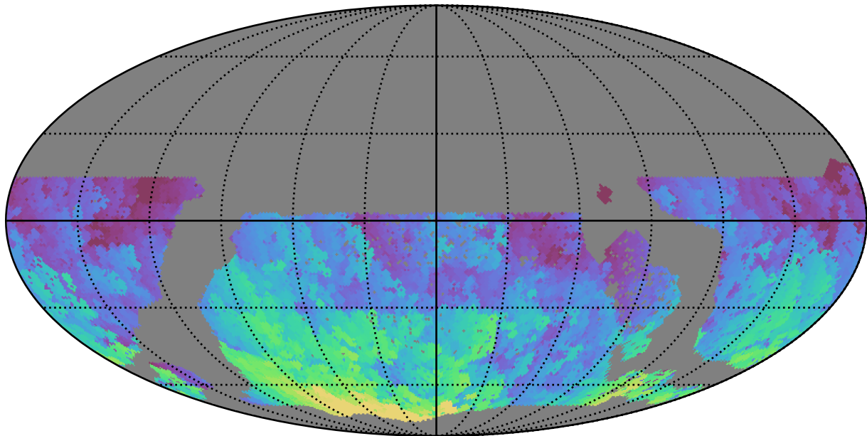
too_5_4v3.4_10yrs WFD u band: Max HA
