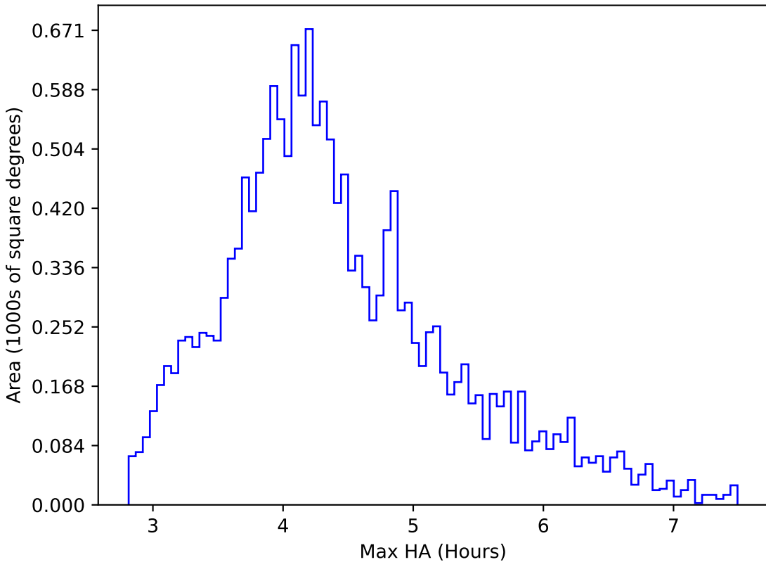
too_5_4v3.4_10yrs WFD r band: Max HA
