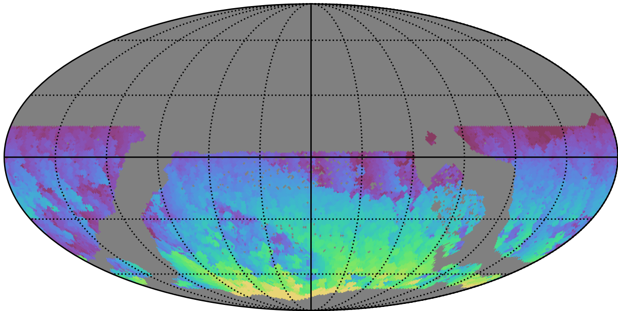
too_5_4v3.4_10yrs WFD i band: Max HA
