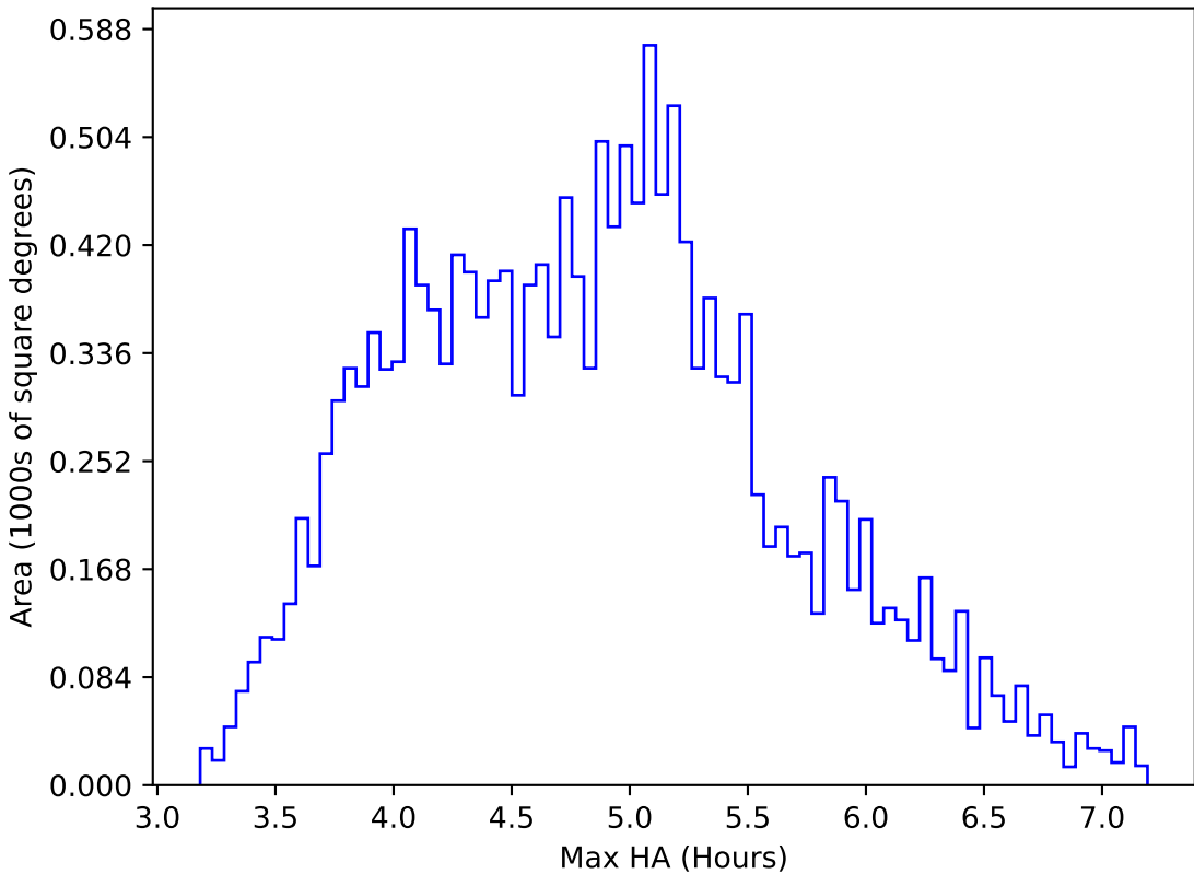
too_5_4v3.4_10yrs WFD i band: Max HA
