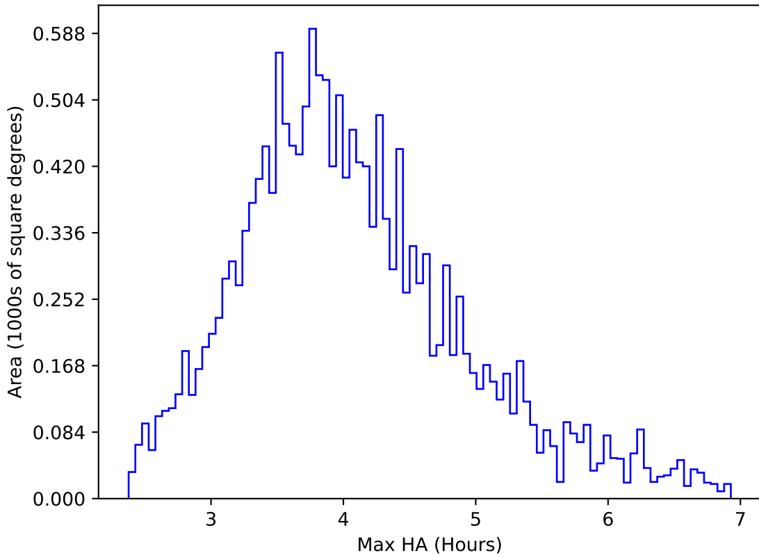
too_5_4v3.4_10yrs WFD g band: Max HA
