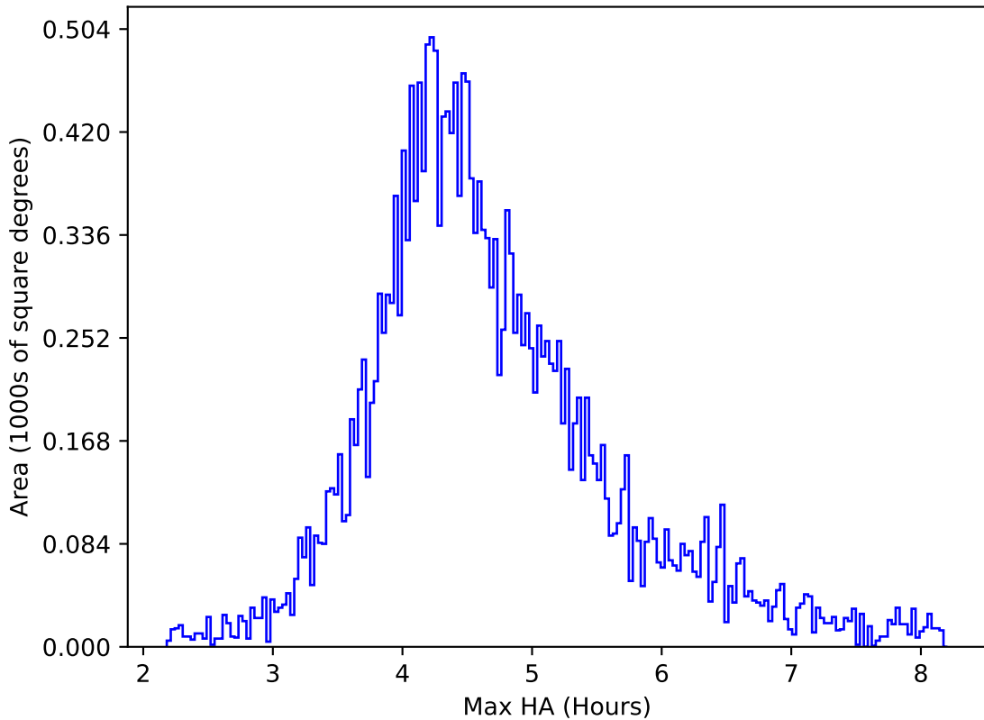
too_5_4v3.4_10yrs All sky y band: Max HA
