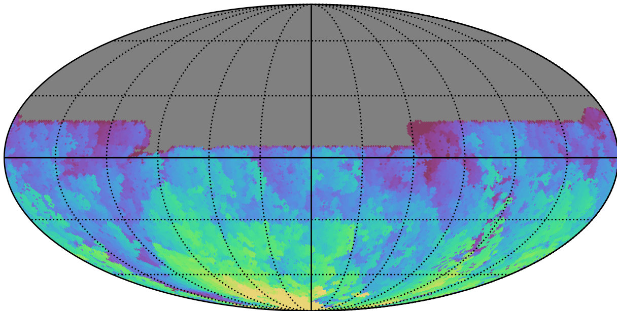
too_5_4v3.4_10yrs All sky u band: Max HA
