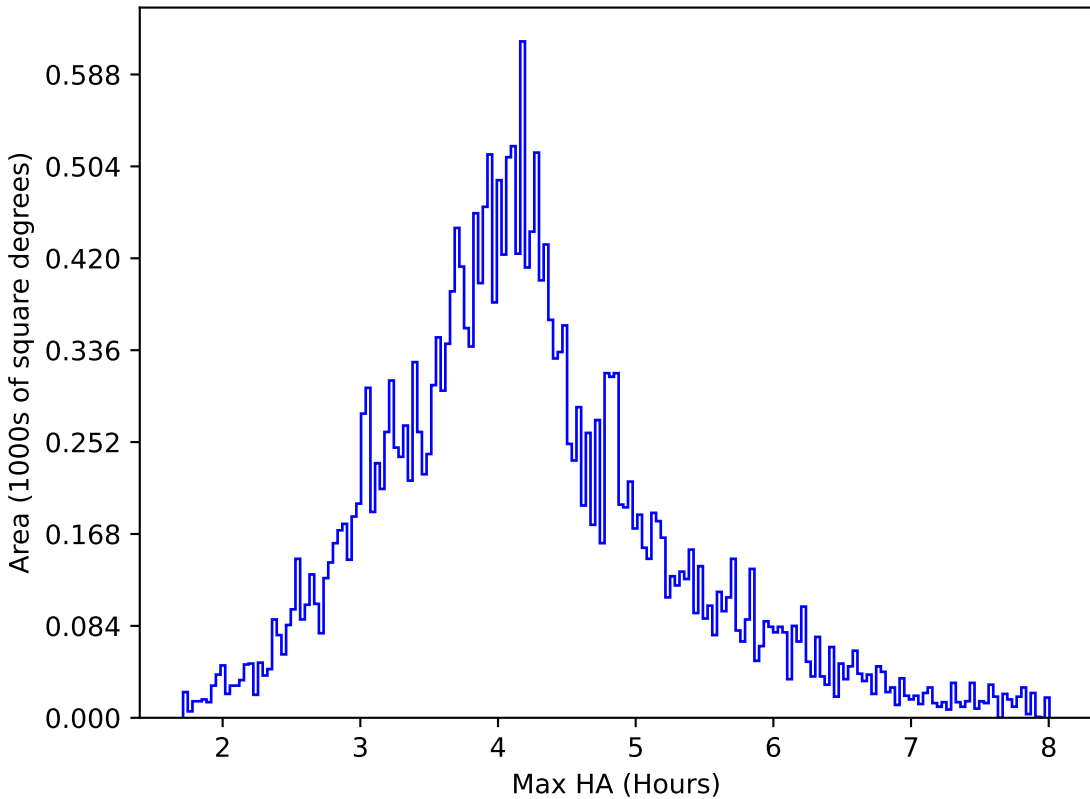
too_5_4v3.4_10yrs All sky r band: Max HA
