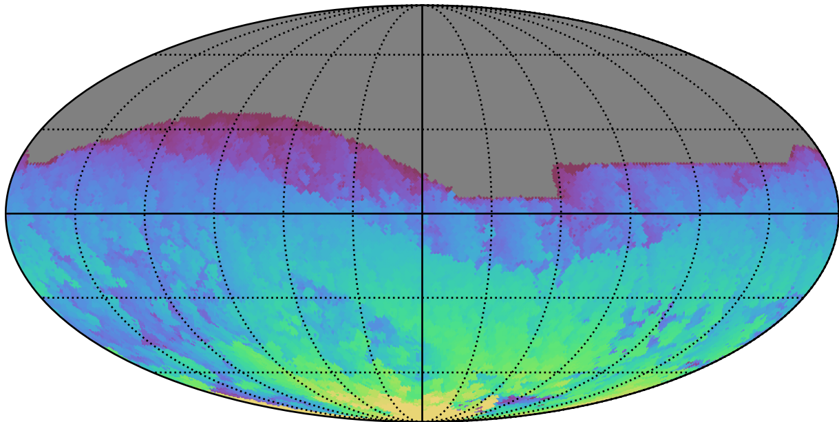
too_5_4v3.4_10yrs All sky i band: Max HA
