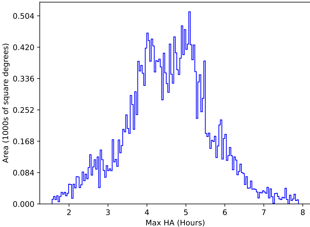
too_5_4v3.4_10yrs All sky i band: Max HA
