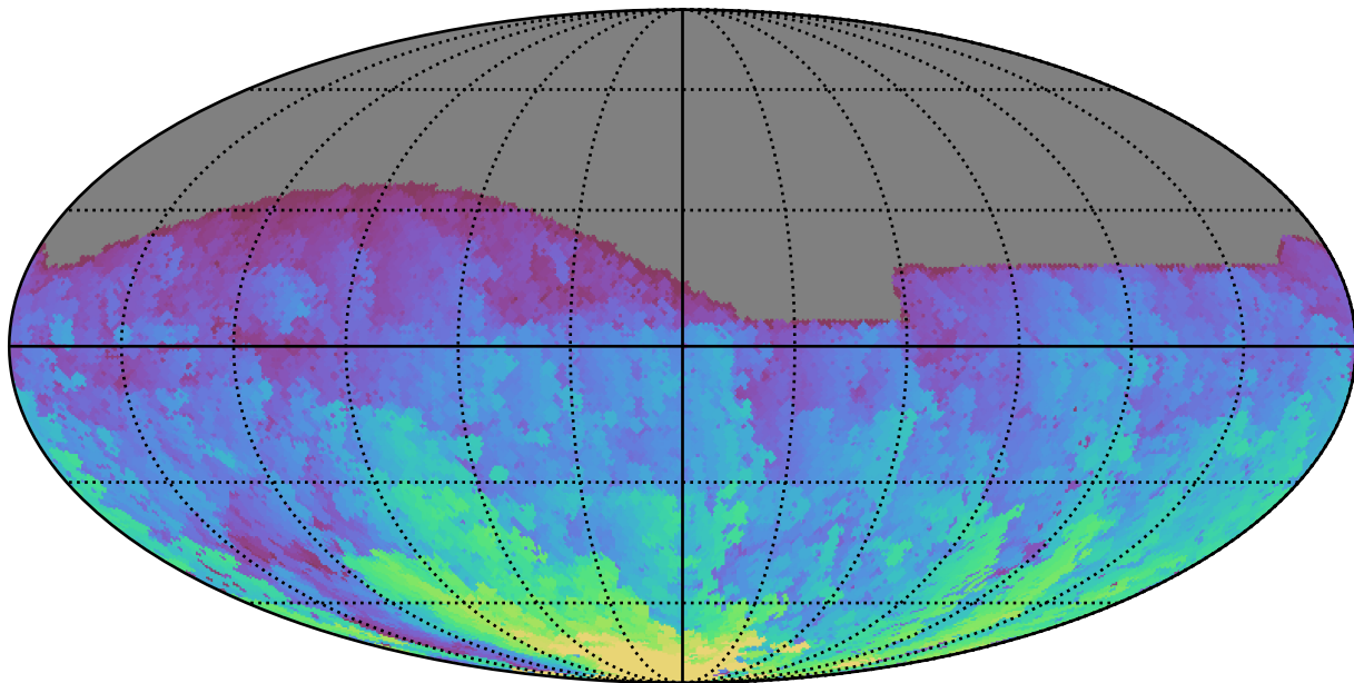
too_5_4v3.4_10yrs All sky g band: Max HA
