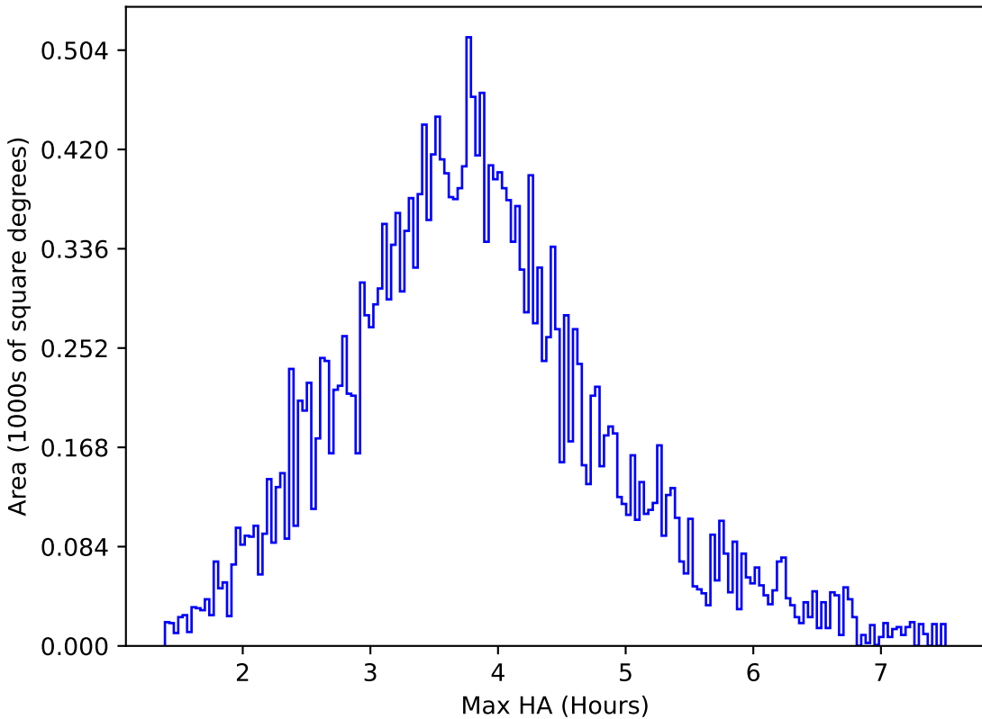
too_5_4v3.4_10yrs All sky g band: Max HA
