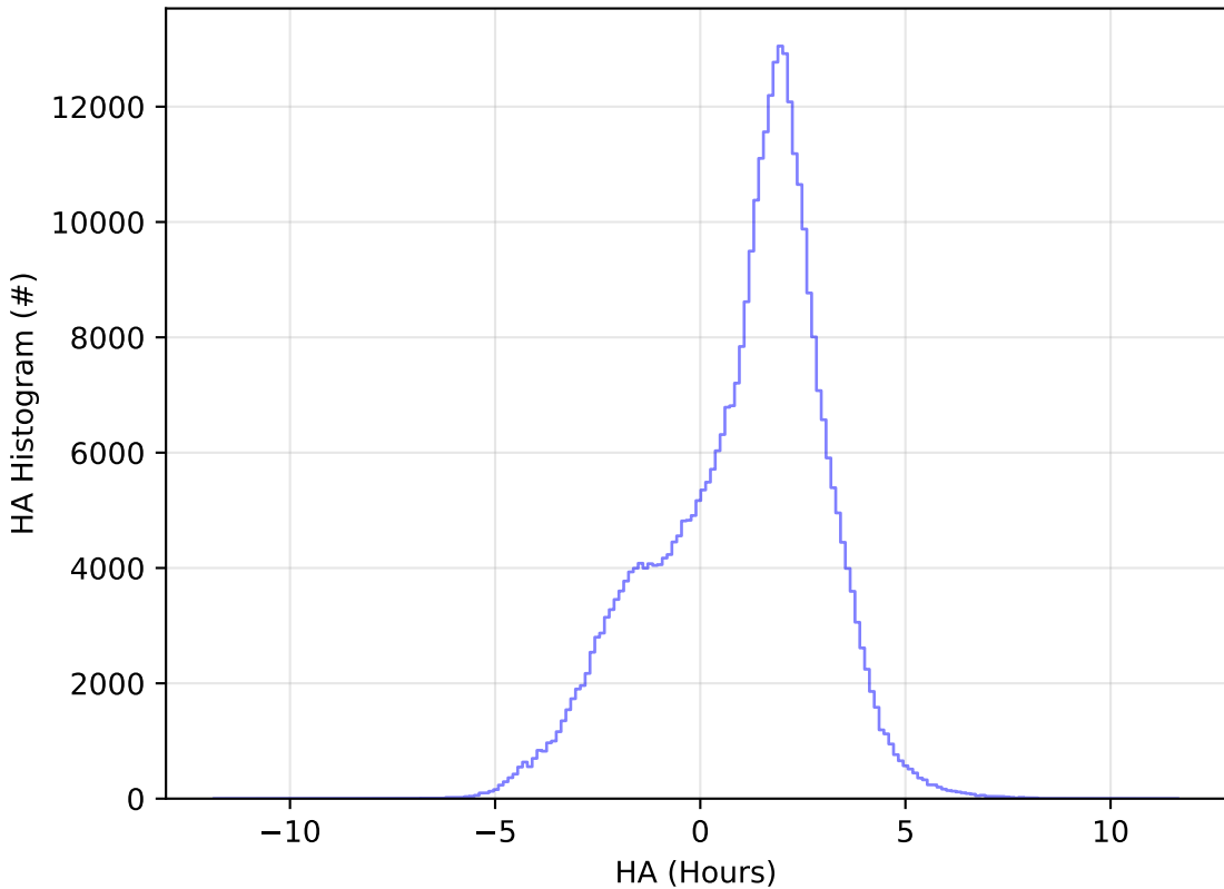
too_5_4v3.4_10yrs WFD y band: HA Histogram
