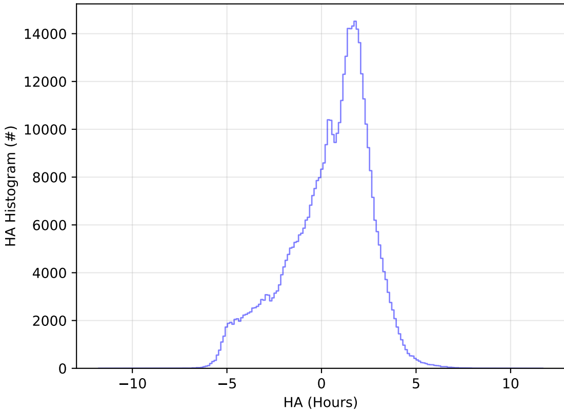
too_5_4v3.4_10yrs WFD r band: HA Histogram
