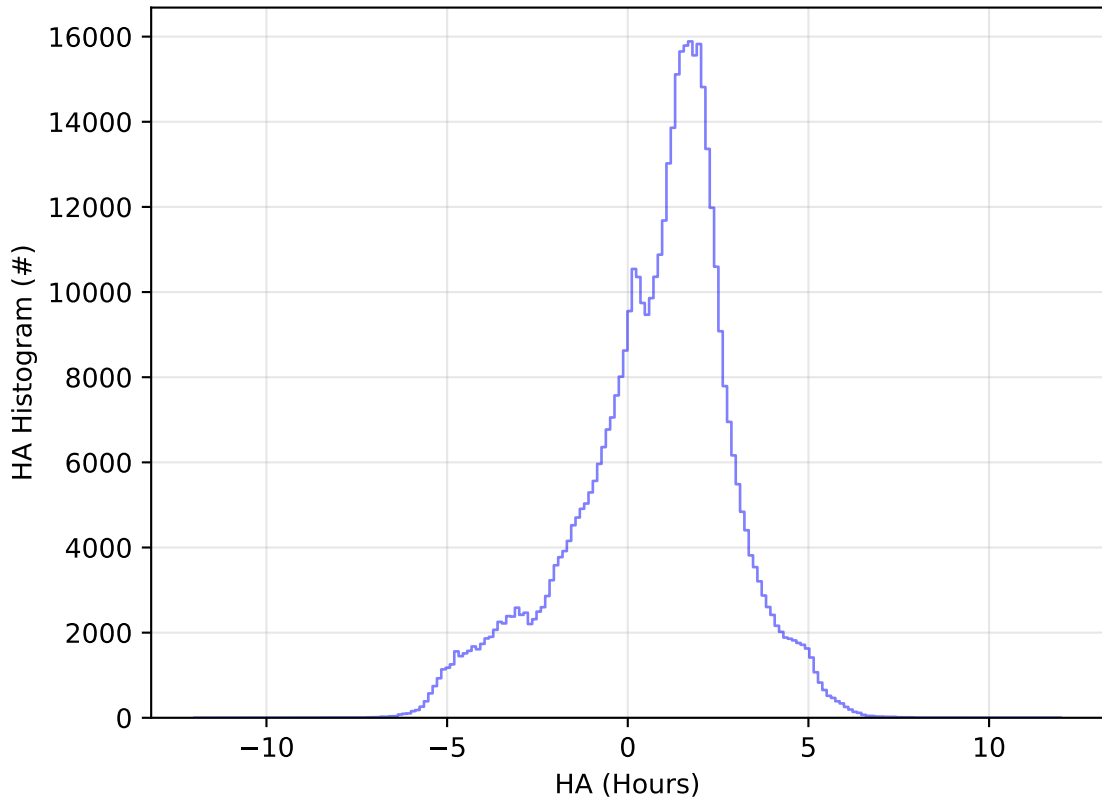
too_5_4v3.4_10yrs WFD i band: HA Histogram
