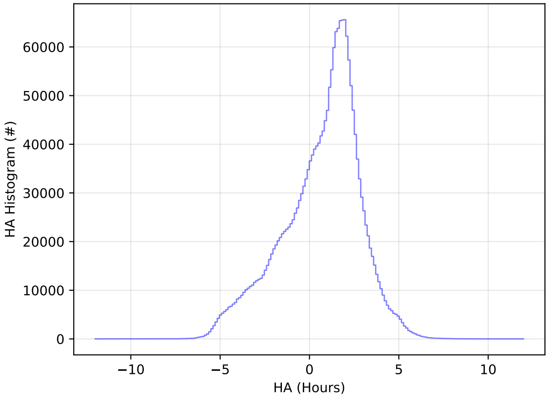
too_5_4v3.4_10yrs WFD all bands: HA Histogram
