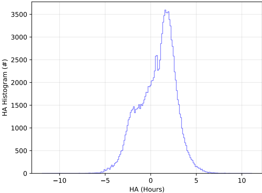
too_5_4v3.4_10yrs All sky u band: HA Histogram
