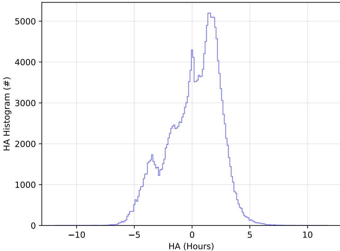
too_5_4v3.4_10yrs All sky g band: HA Histogram
