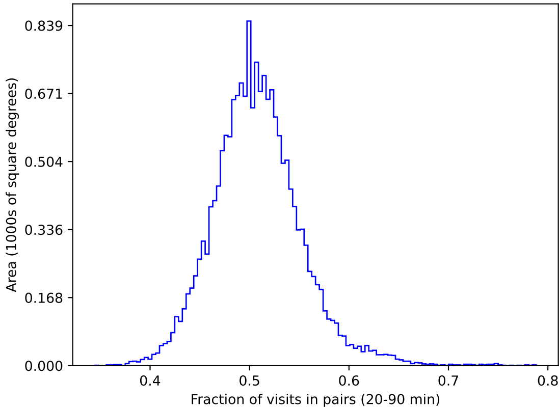
too_5_4v3.4_10yrs gri WFD: Fraction of visits in pairs (20-90 min)
