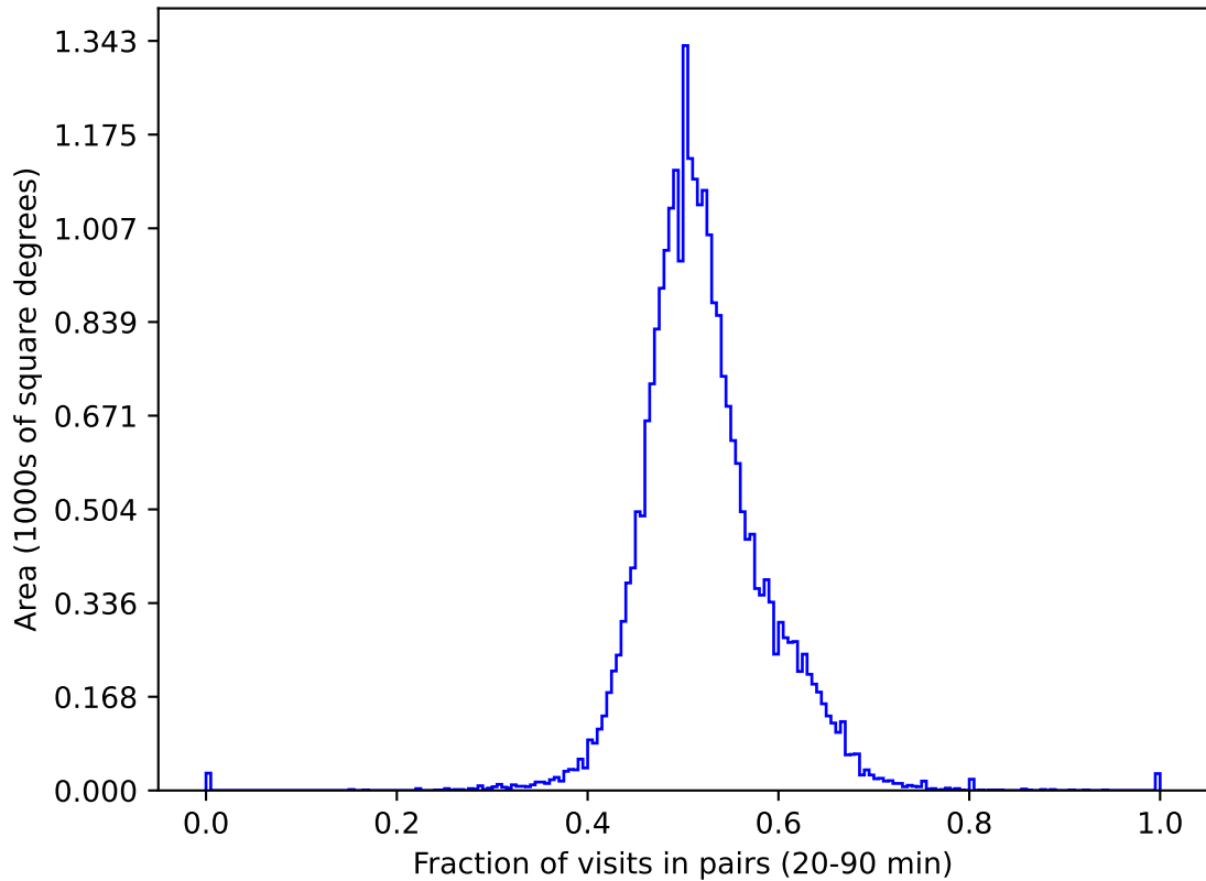
too_5_4v3.4_10yrs gri All sky: Fraction of visits in pairs (20-90 min)
