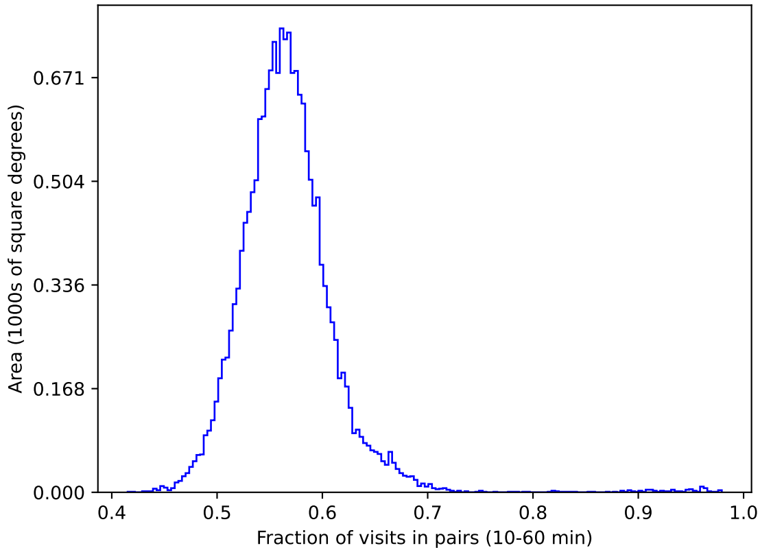
too_5_4v3.4_10yrs gri WFD: Fraction of visits in pairs (10-60 min)
