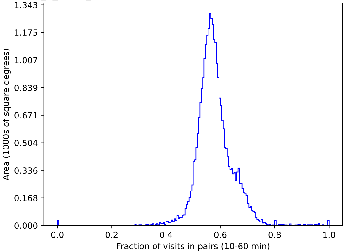
too_5_4v3.4_10yrs gri All sky: Fraction of visits in pairs (10-60 min)
