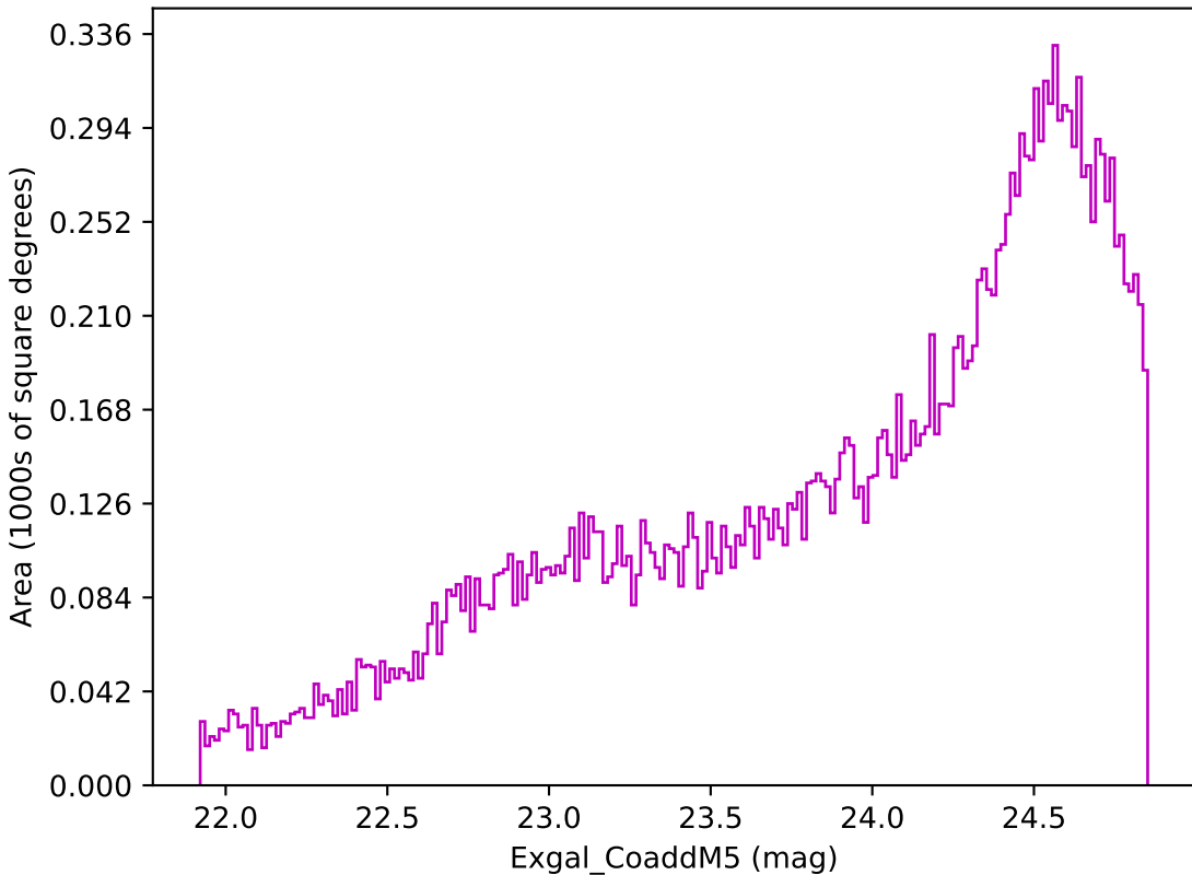
too_5_4v3.4_10yrs Yr 3-4 z band: Exgal_CoaddM5
