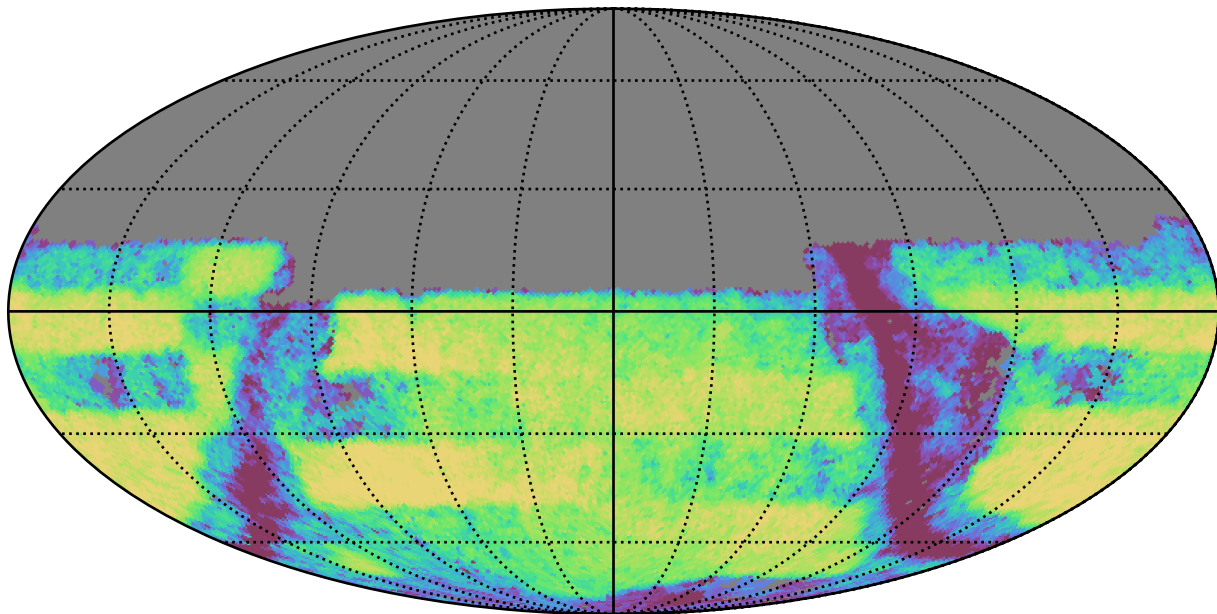
too_5_4v3.4_10yrs Yr 3-4 y band: Exgal_CoaddM5
