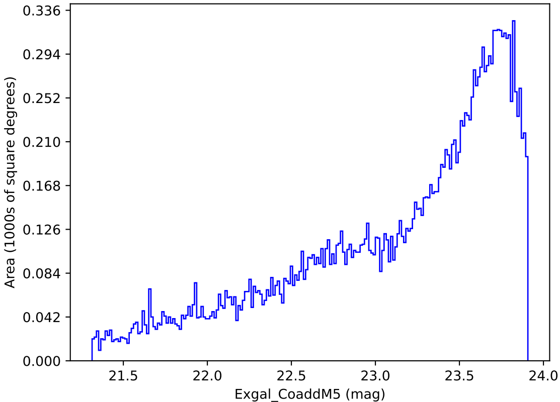
too_5_4v3.4_10yrs Yr 3-4 y band: Exgal_CoaddM5
