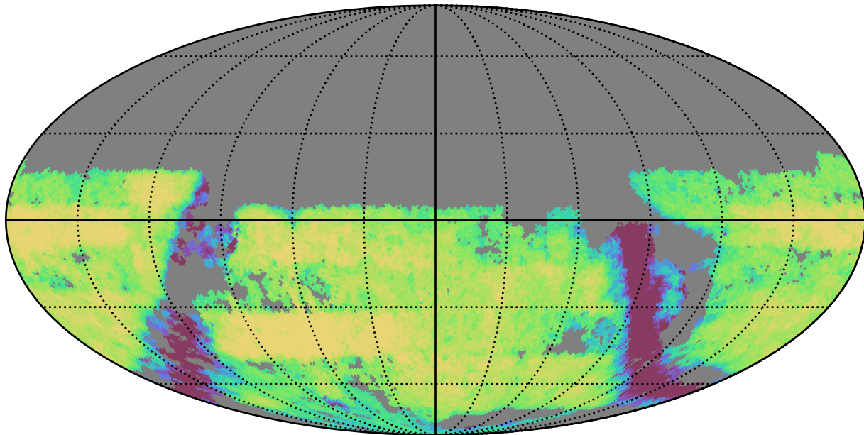
too_5_4v3.4_10yrs Yr 3-4 u band: Exgal_CoaddM5
