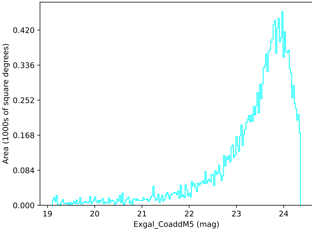
too_5_4v3.4_10yrs Yr 3-4 u band: Exgal_CoaddM5
