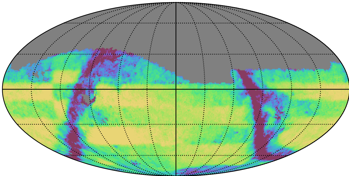
too_5_4v3.4_10yrs Yr 3-4 r band: Exgal_CoaddM5
